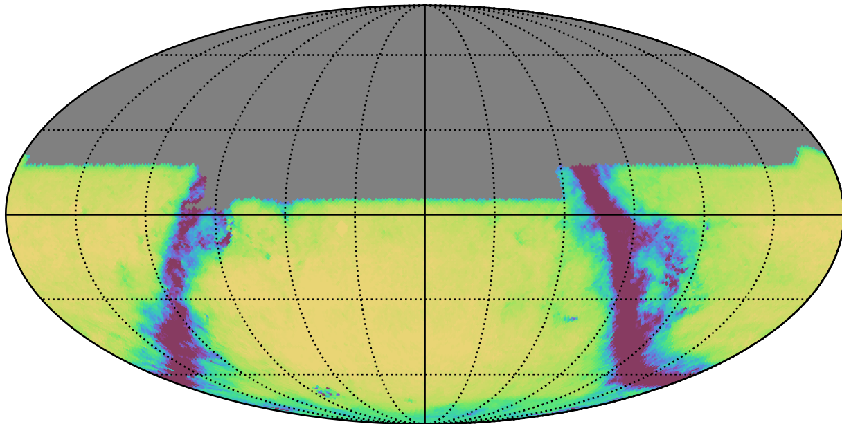
too_ignore_100_4v3.4_10yrs All sky u band: Exgal_CoaddM5
