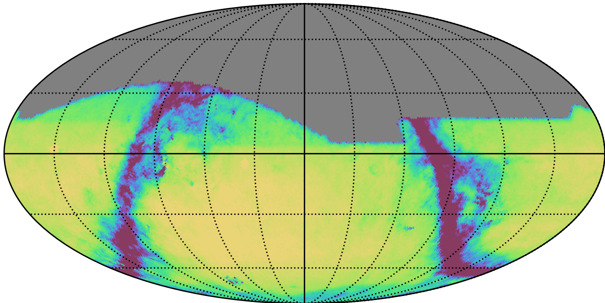
too_ignore_100_4v3.4_10yrs All sky g band: Exgal_CoaddM5
