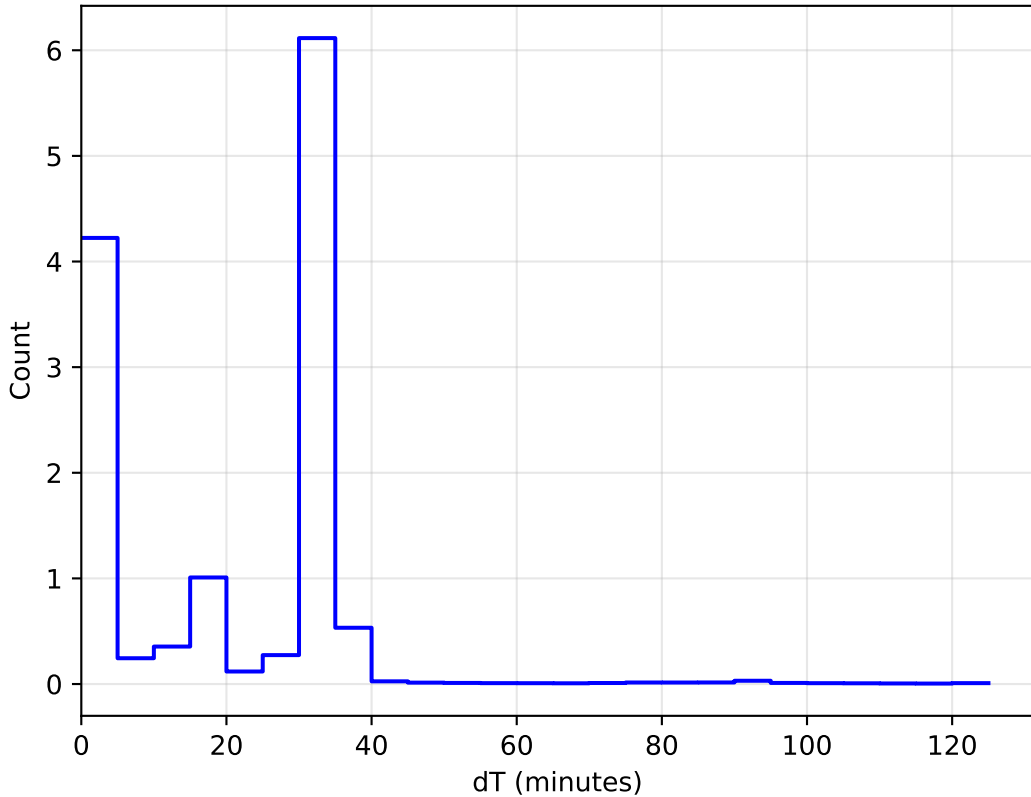
too_ignore_100_4v3.4_10yrs All sky: DeltaT Histogram
