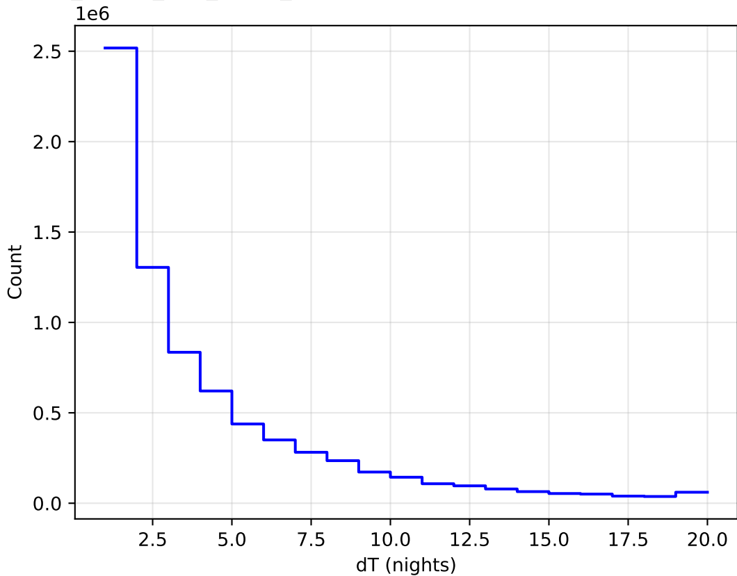
too_ignore_100_4v3.4_10yrs WFD all bands: DeltaNight Histogram
