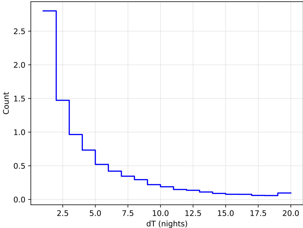
too_ignore_100_4v3.4_10yrs All sky all bands: DeltaNight Histogram 1e6
