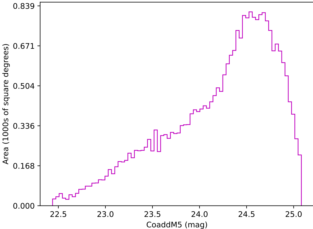
too_ignore_100_4v3.4_10yrs Yr 3-4 z band: CoaddM5
