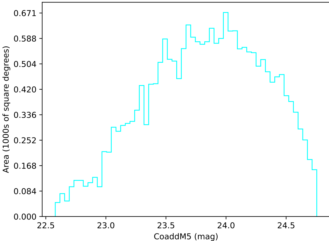
too_ignore_100_4v3.4_10yrs Yr 3-4 u band: CoaddM5
