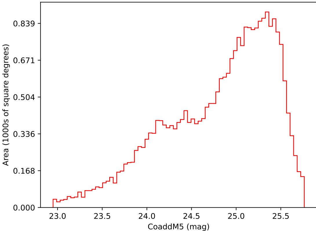
too_ignore_100_4v3.4_10yrs Yr 3-4 i band: CoaddM5
