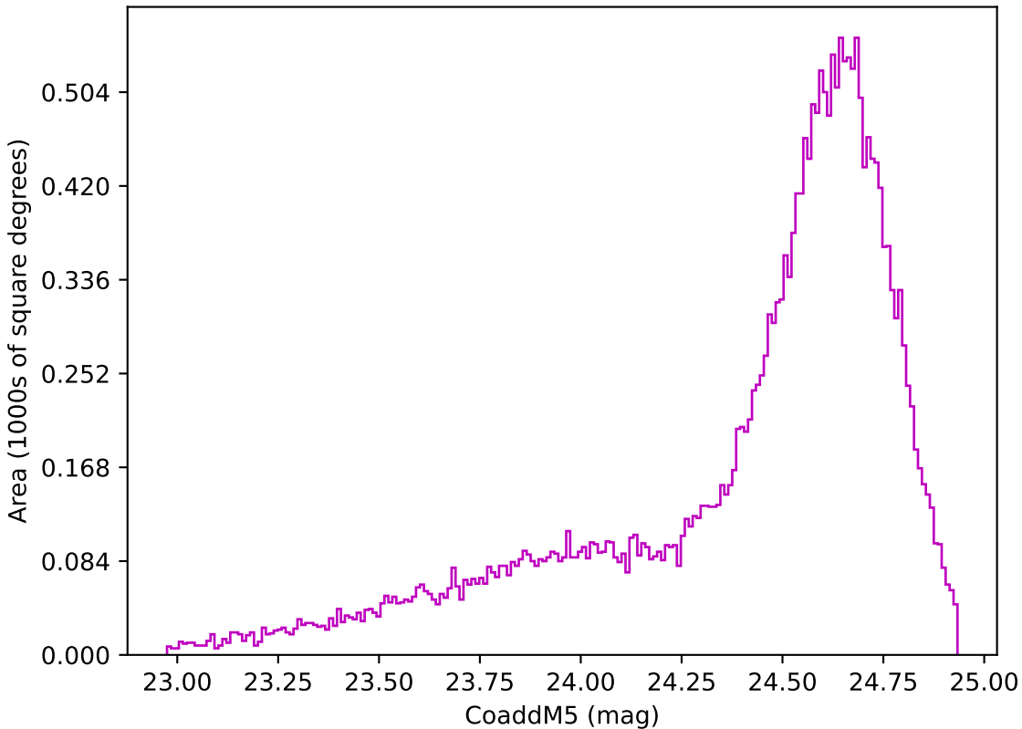
too_ignore_100_4v3.4_10yrs Yr 1 z band: CoaddM5
