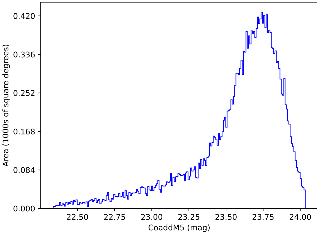
too_ignore_100_4v3.4_10yrs Yr 1 y band: CoaddM5
