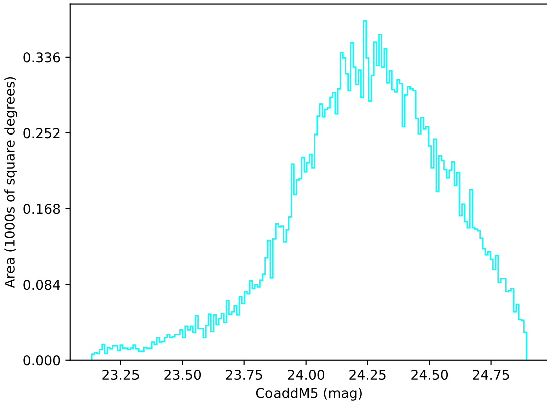
too_ignore_100_4v3.4_10yrs Yr 1 u band: CoaddM5
