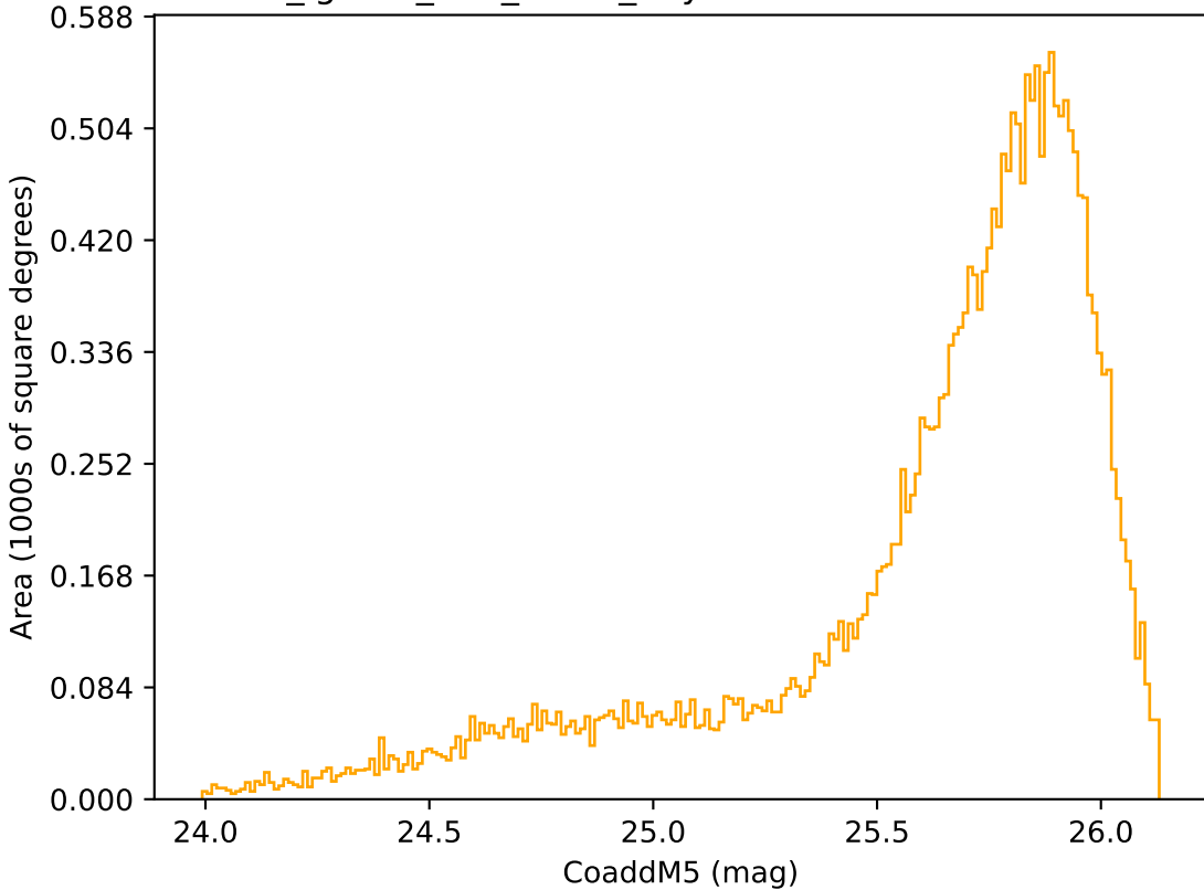
too_ignore_100_4v3.4_10yrs Yr 1 r band: CoaddM5
