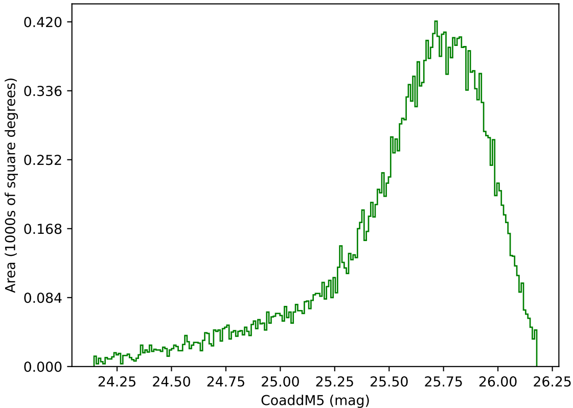
too_ignore_100_4v3.4_10yrs Yr 1 g band: CoaddM5
