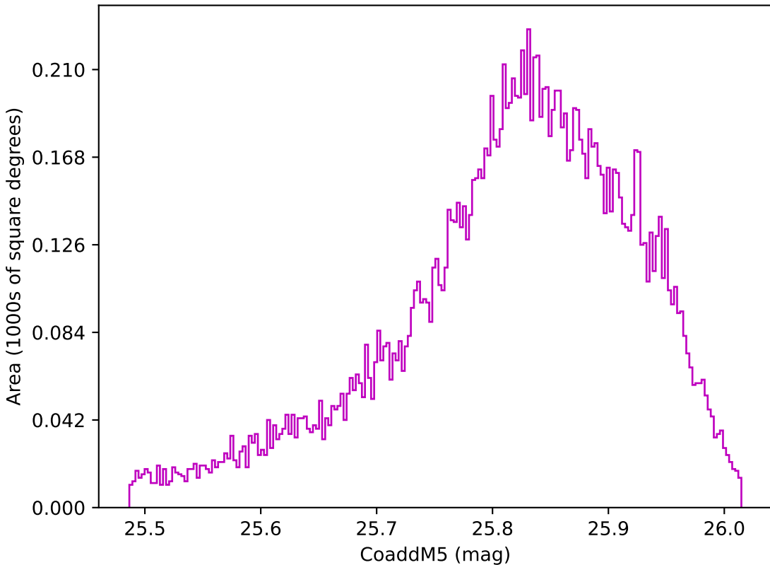
too_ignore_100_4v3.4_10yrs WFD z band: CoaddM5
