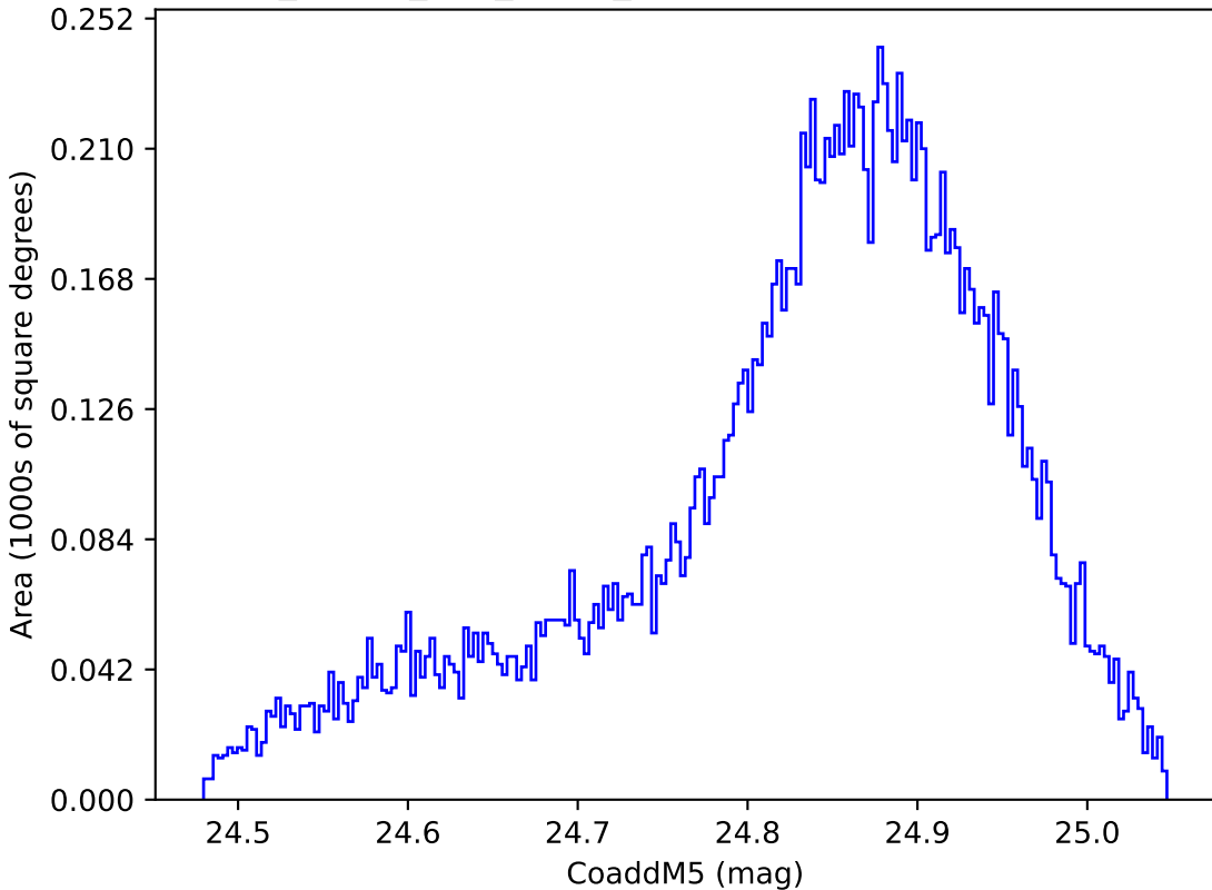
too_ignore_100_4v3.4_10yrs WFD y band: CoaddM5
