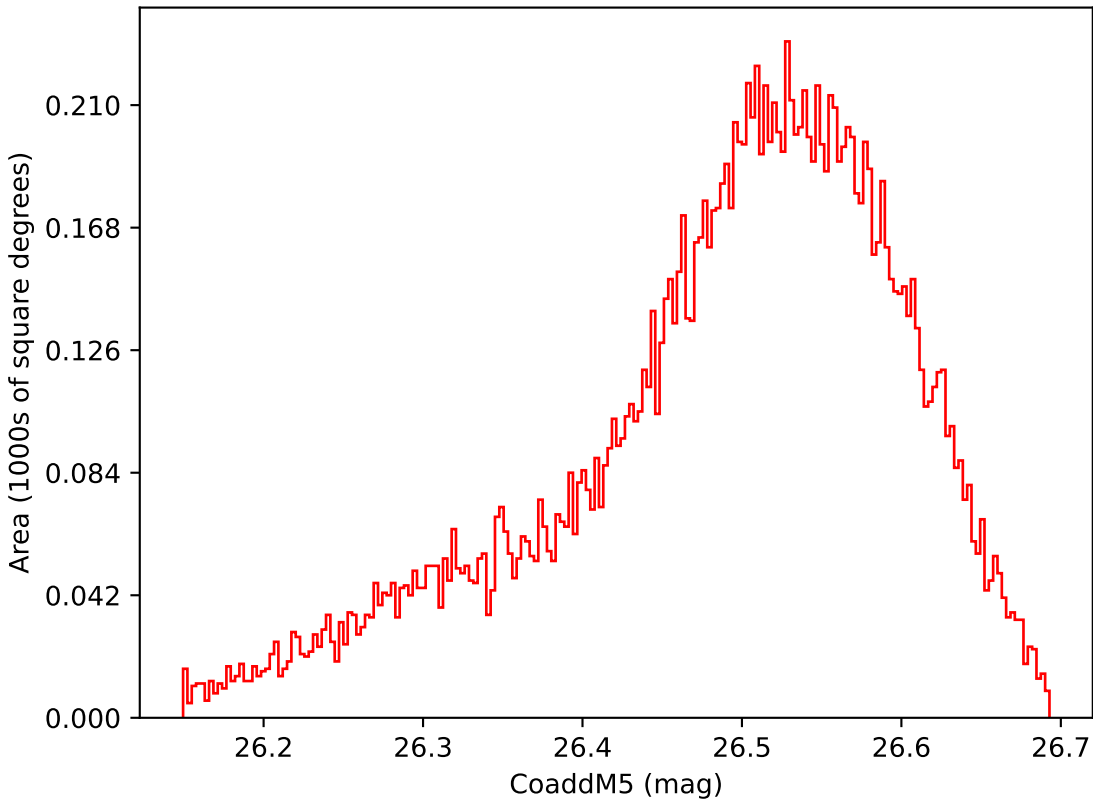
too_ignore_100_4v3.4_10yrs WFD i band: CoaddM5
