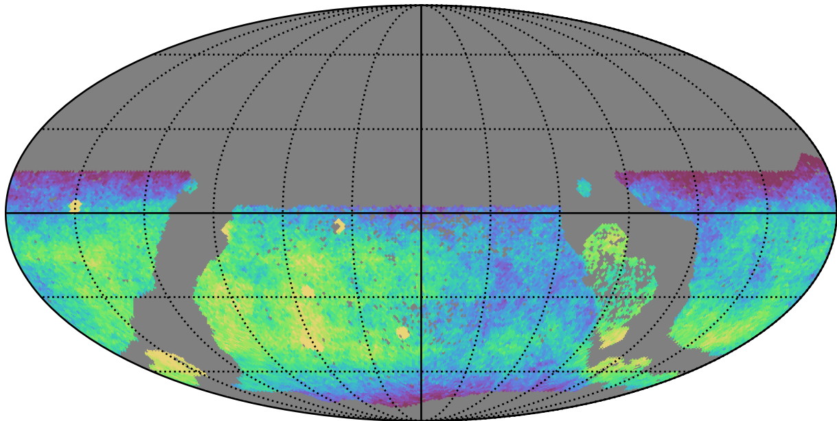
too_ignore_100_4v3.4_10yrs WFD g band: CoaddM5
