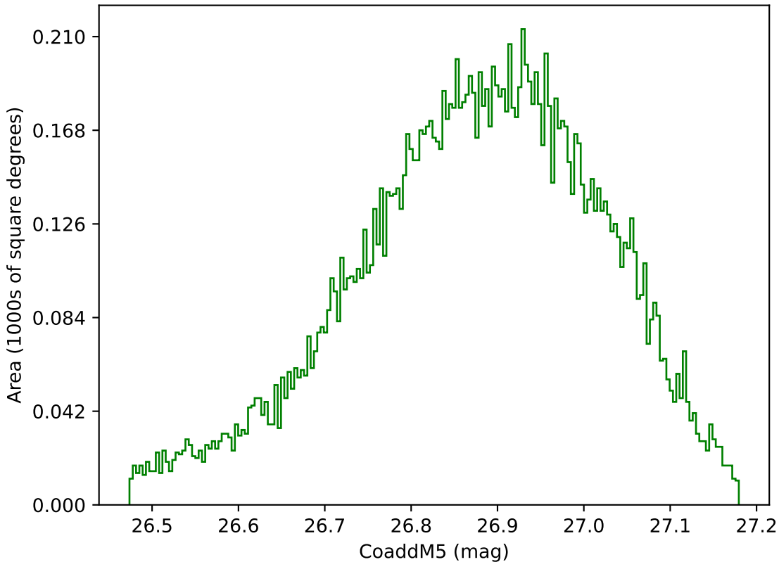
too_ignore_100_4v3.4_10yrs WFD g band: CoaddM5
