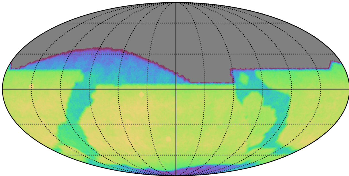
too_ignore_100_4v3.4_10yrs All sky z band: CoaddM5
