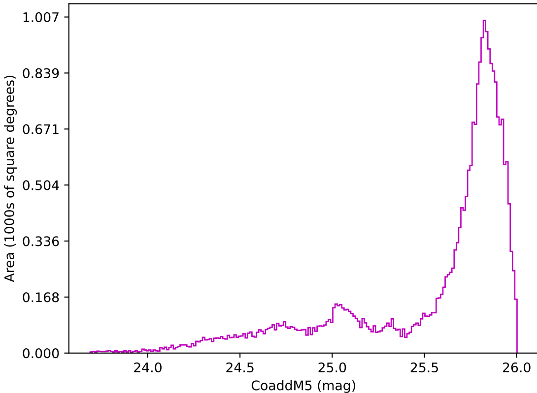
too_ignore_100_4v3.4_10yrs All sky z band: CoaddM5
