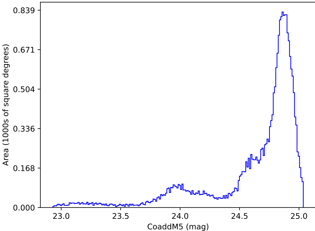
too_ignore_100_4v3.4_10yrs All sky y band: CoaddM5
