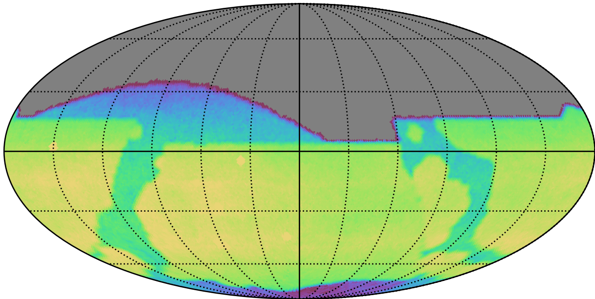
too_ignore_100_4v3.4_10yrs All sky r band: CoaddM5
