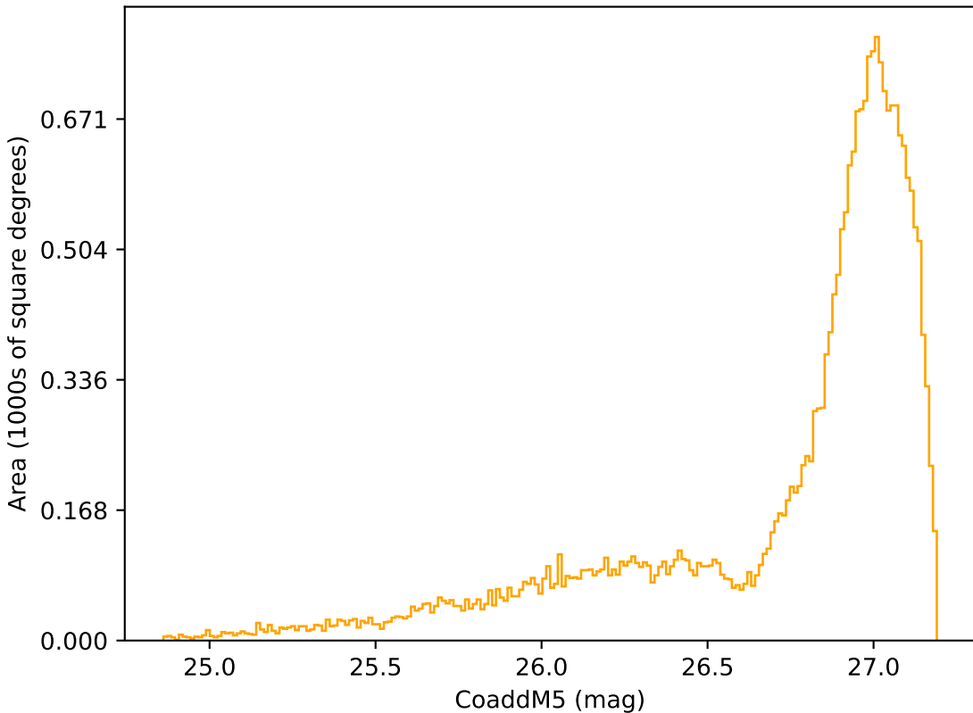
too_ignore_100_4v3.4_10yrs All sky r band: CoaddM5
