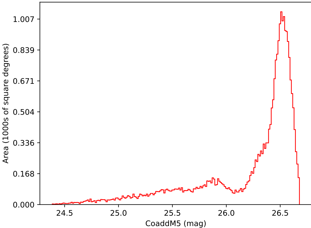
too_ignore_100_4v3.4_10yrs All sky i band: CoaddM5
