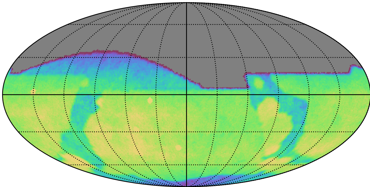
too_ignore_100_4v3.4_10yrs All sky g band: CoaddM5
