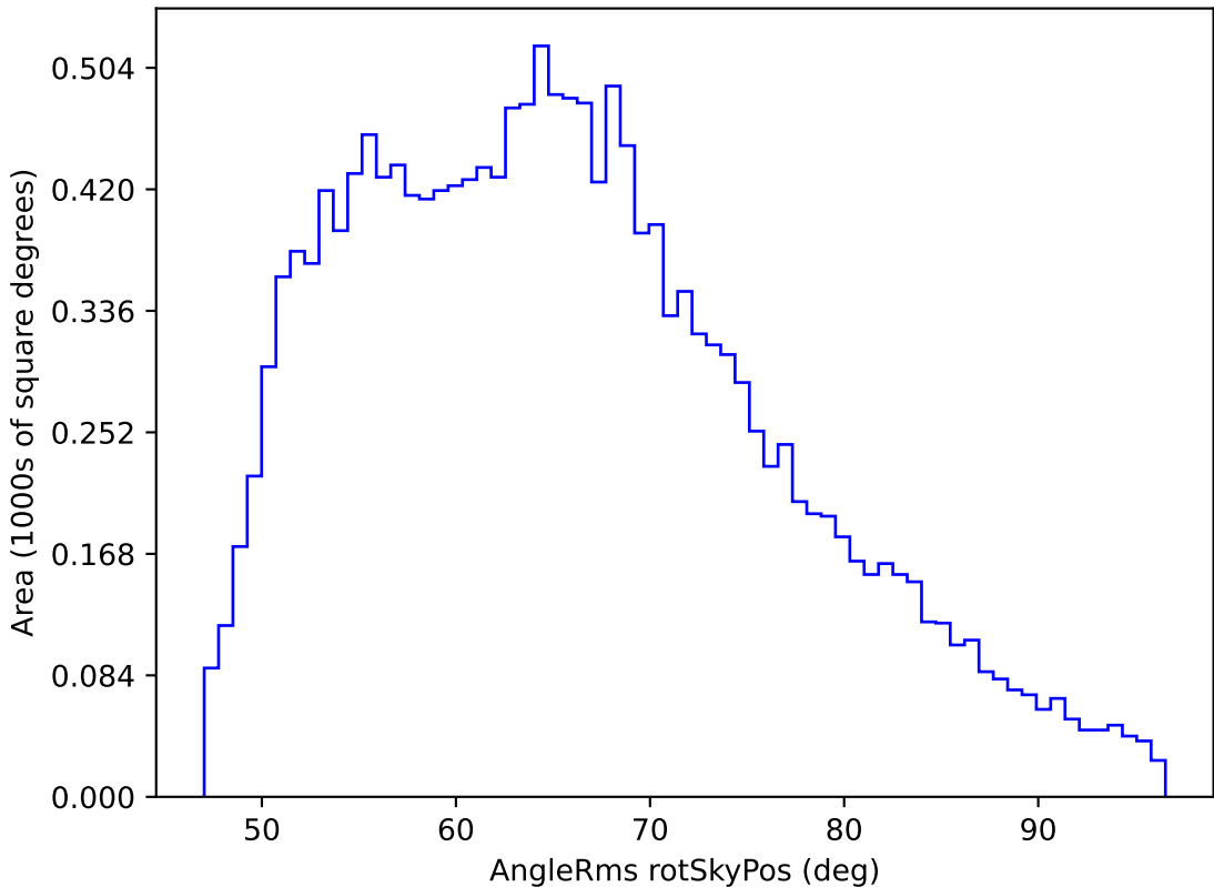
too_ignore_100_4v3.4_10yrs WFD z band: AngleRms rotSkyPos
