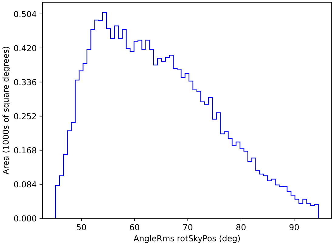
too_ignore_100_4v3.4_10yrs WFD u band: AngleRms rotSkyPos
