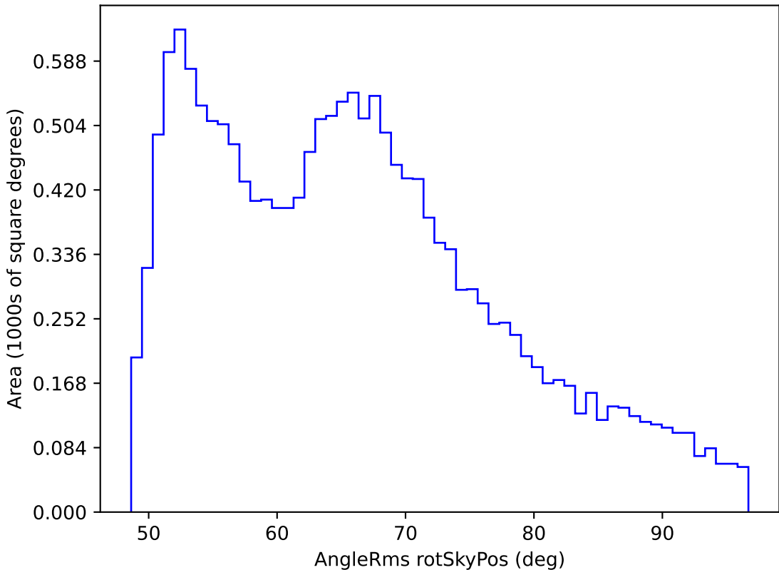
too_ignore_100_4v3.4_10yrs WFD r band: AngleRms rotSkyPos
