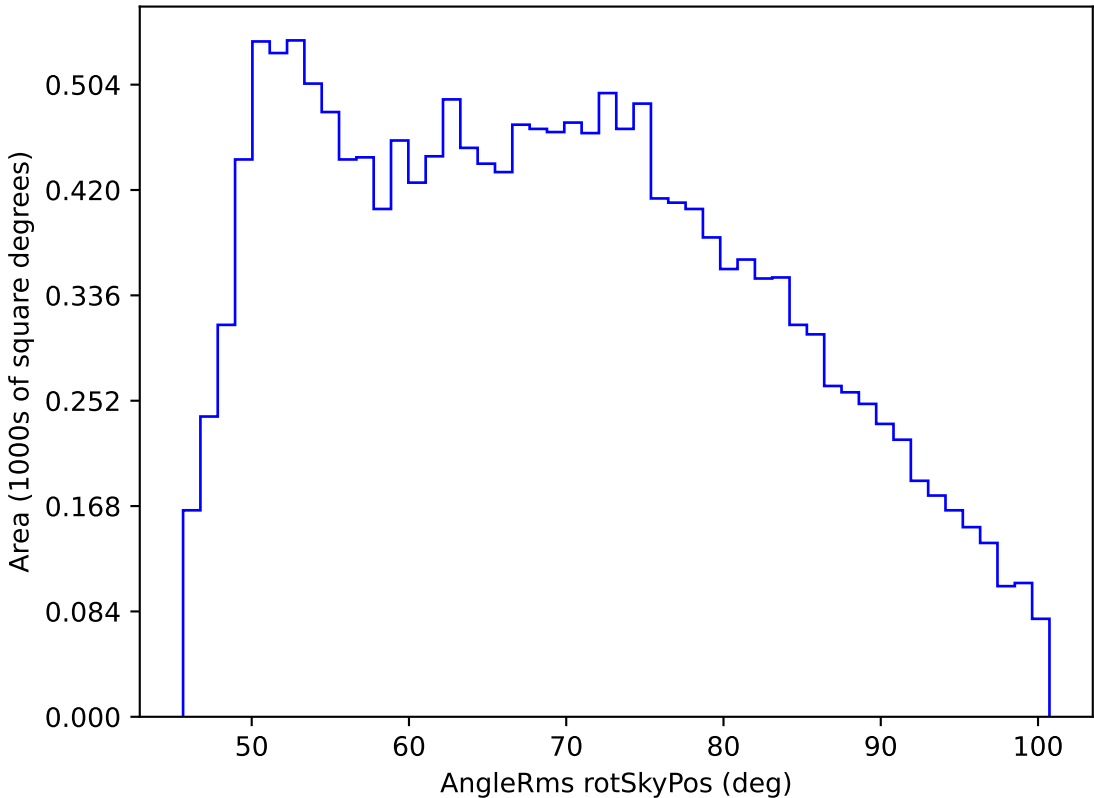
too_ignore_100_4v3.4_10yrs WFD g band: AngleRms rotSkyPos
