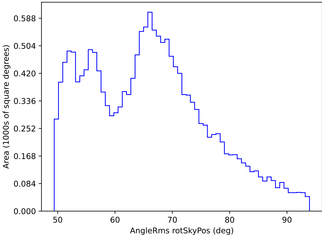
too_ignore_100_4v3.4_10yrs WFD all bands: AngleRms rotSkyPos
