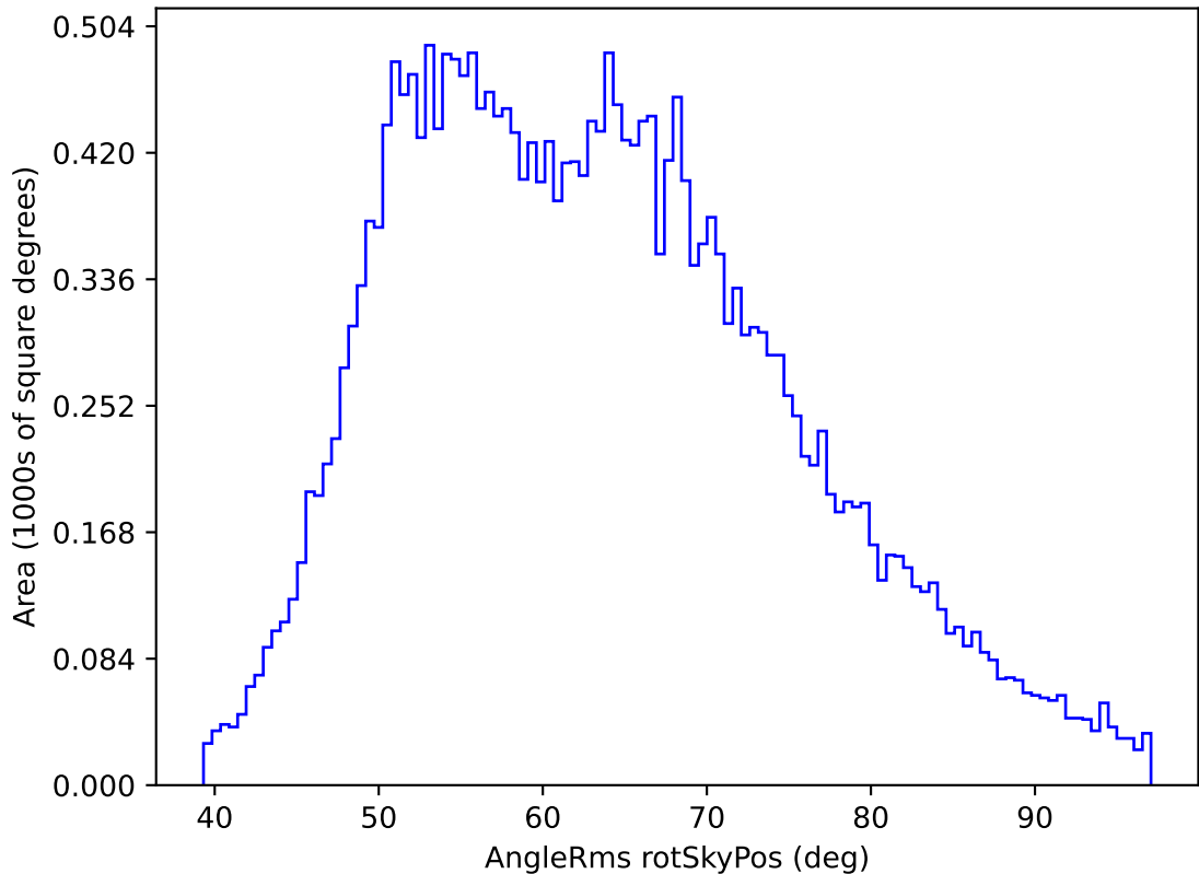
too_ignore_100_4v3.4_10yrs All sky z band: AngleRms rotSkyPos
