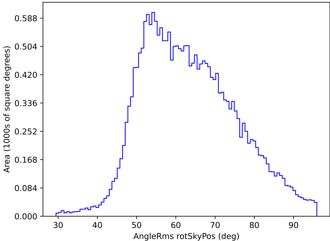
too_ignore_100_4v3.4_10yrs All sky u band: AngleRms rotSkyPos
