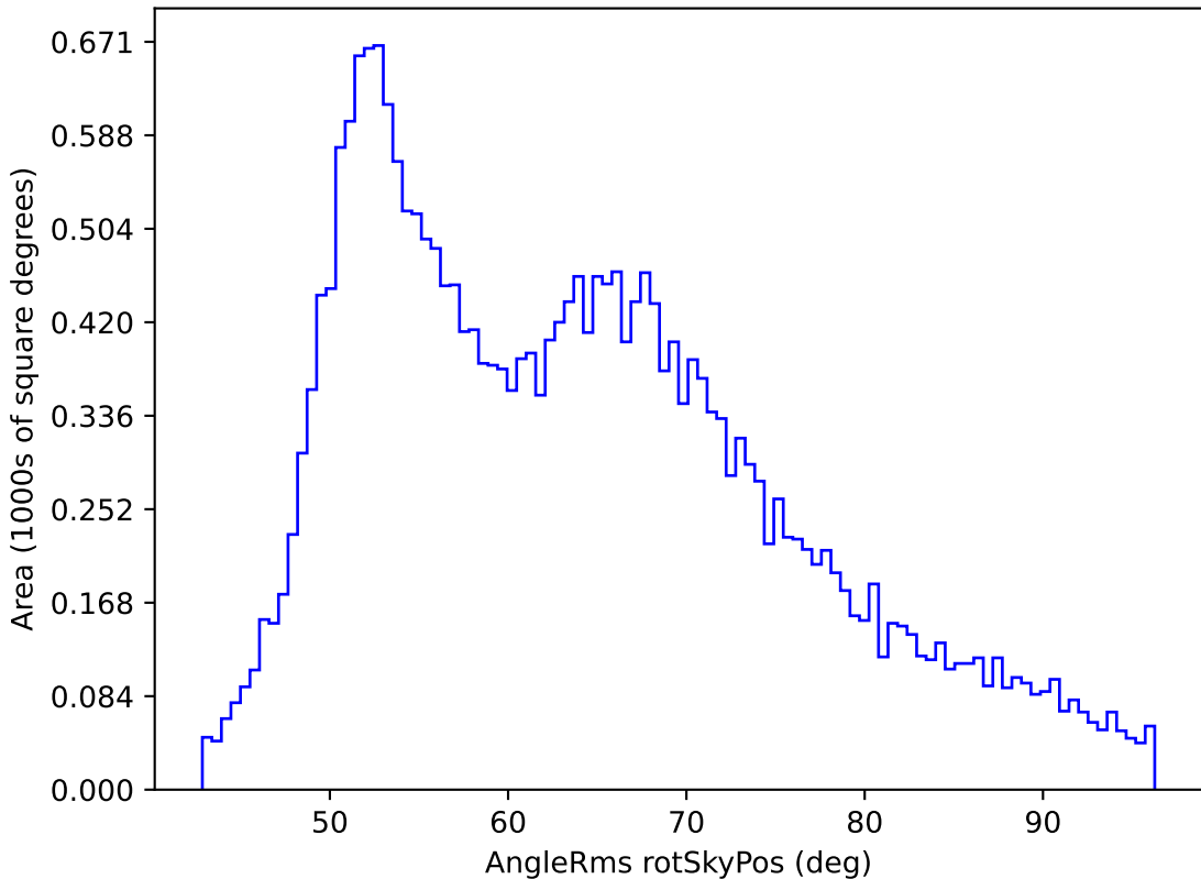
too_ignore_100_4v3.4_10yrs All sky r band: AngleRms rotSkyPos
