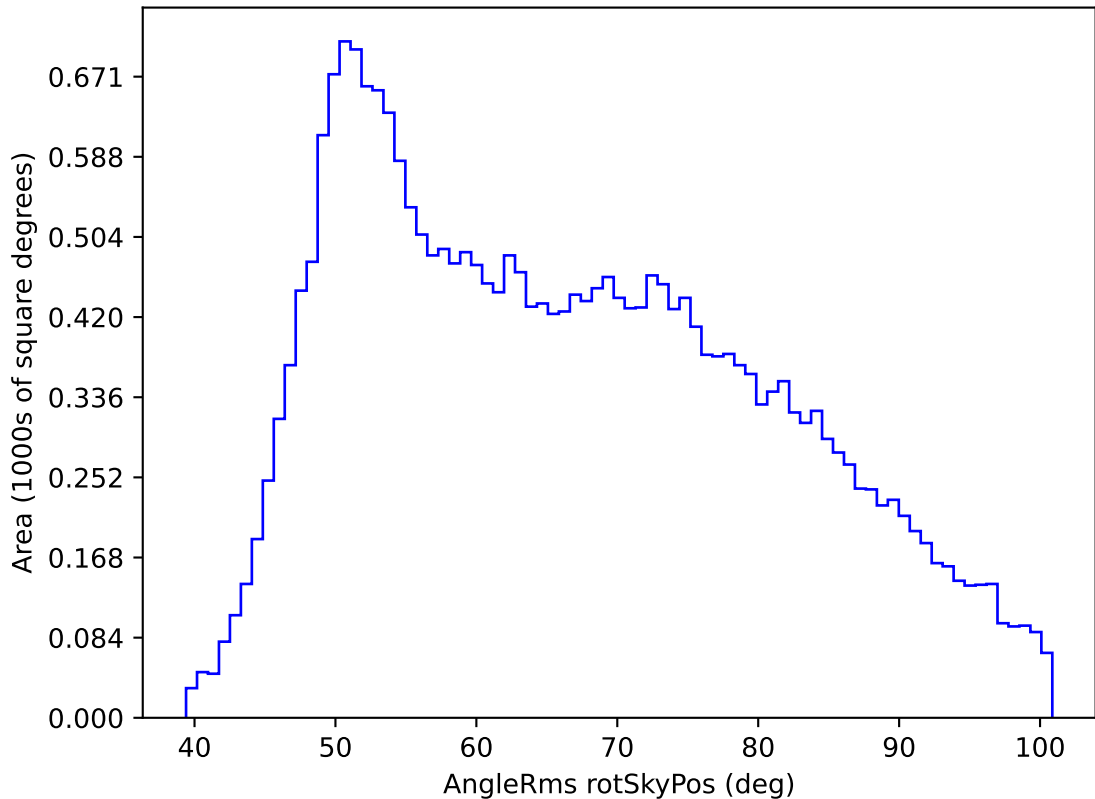
too_ignore_100_4v3.4_10yrs All sky g band: AngleRms rotSkyPos
