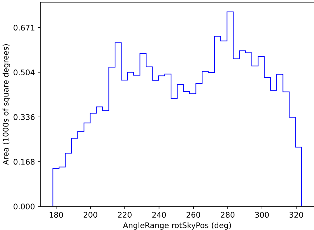
too_ignore_100_4v3.4_10yrs WFD u band: AngleRange rotSkyPos
