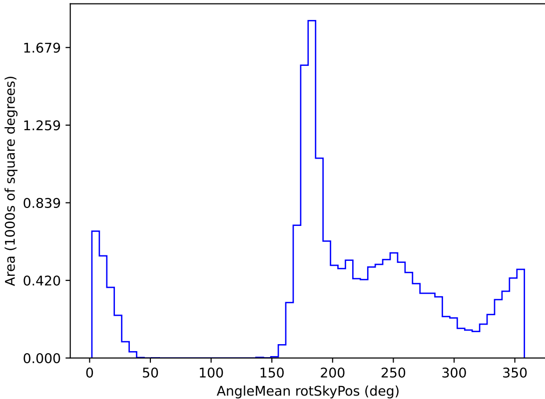
too_ignore_100_4v3.4_10yrs WFD z band: AngleMean rotSkyPos
