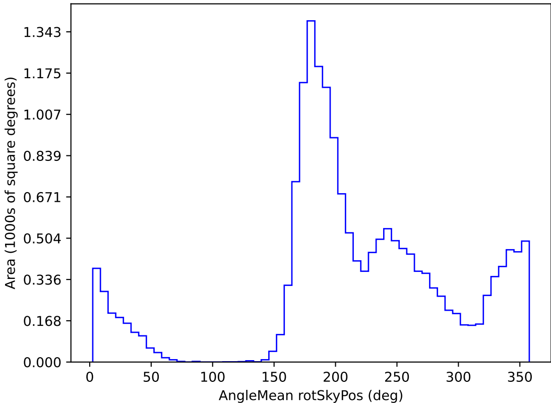
too_ignore_100_4v3.4_10yrs WFD u band: AngleMean rotSkyPos
