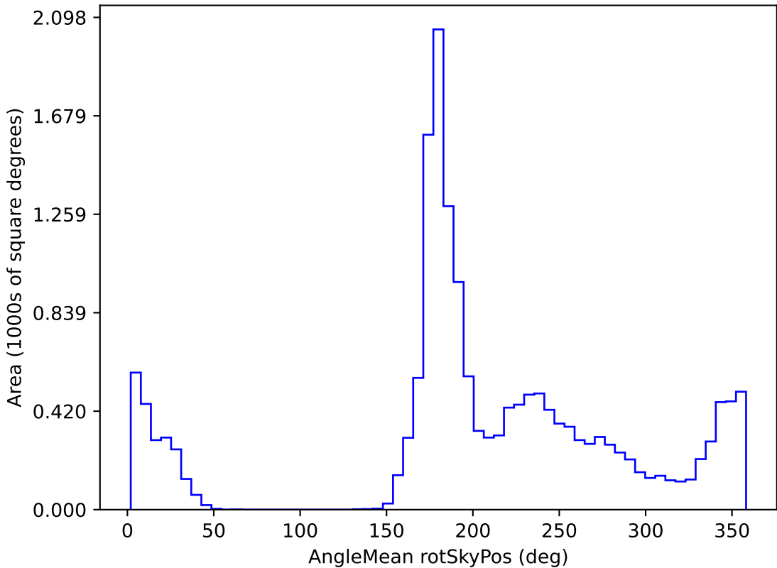
too_ignore_100_4v3.4_10yrs WFD r band: AngleMean rotSkyPos
