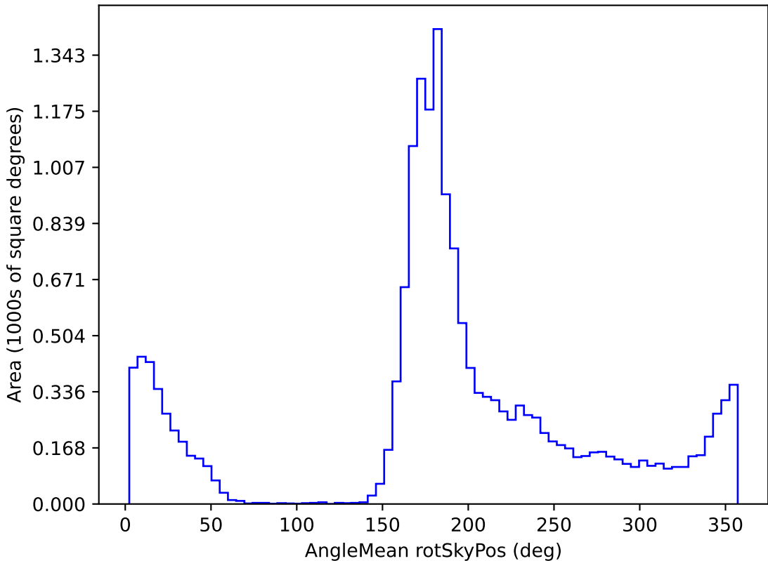
too_ignore_100_4v3.4_10yrs WFD g band: AngleMean rotSkyPos
