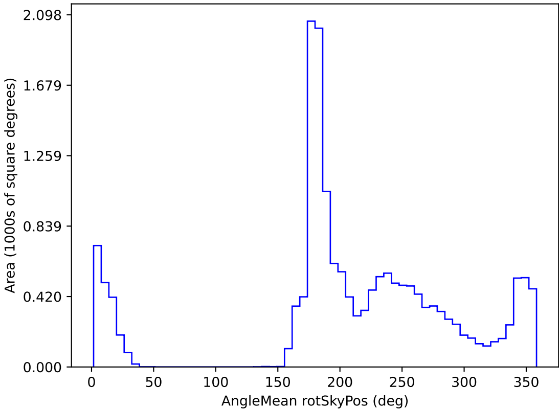
too_ignore_100_4v3.4_10yrs WFD all bands: AngleMean rotSkyPos
