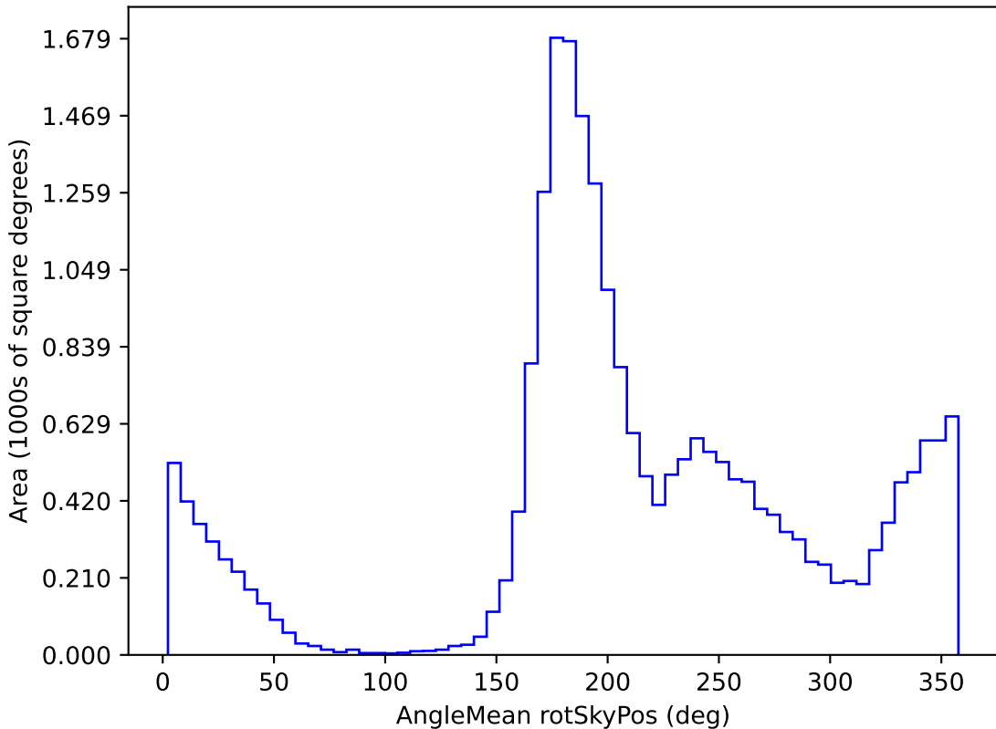
too_ignore_100_4v3.4_10yrs All sky u band: AngleMean rotSkyPos
