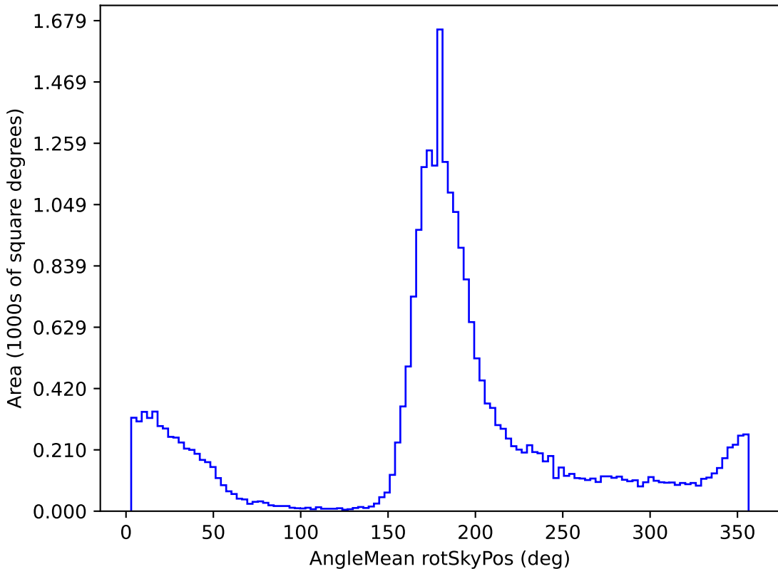
too_ignore_100_4v3.4_10yrs All sky g band: AngleMean rotSkyPos
