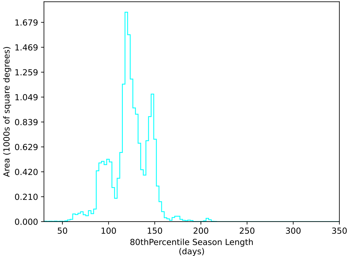
too_ignore_100_4v3.4_10yrs WFD u band: 80thPercentile Season Length
