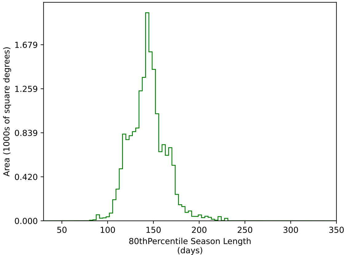
too_ignore_100_4v3.4_10yrs WFD g band: 80thPercentile Season Length
