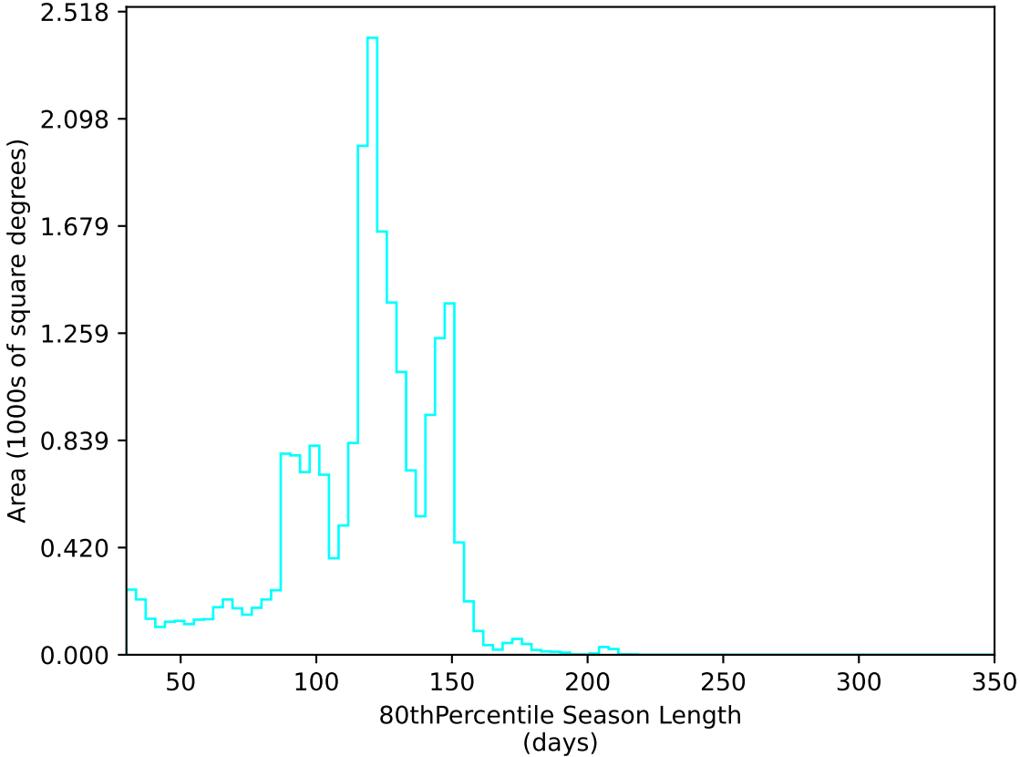
too_ignore_100_4v3.4_10yrs All sky u band: 80thPercentile Season Length
