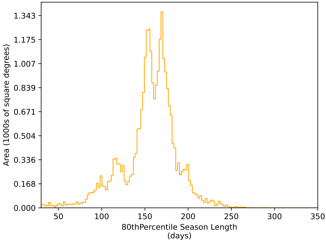
too_ignore_100_4v3.4_10yrs All sky r band: 80thPercentile Season Length
