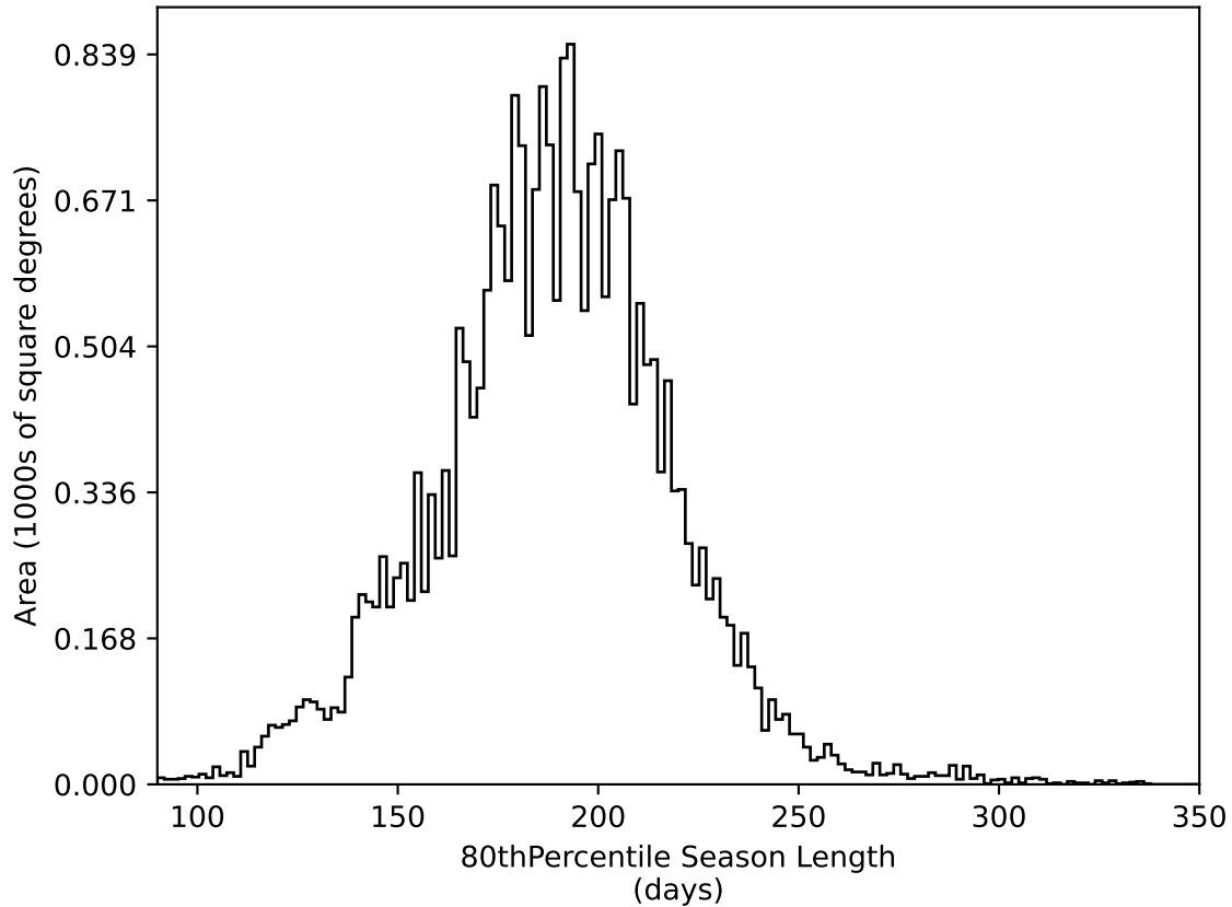
too_ignore_100_4v3.4_10yrs All sky all bands: 80thPercentile Season Length
