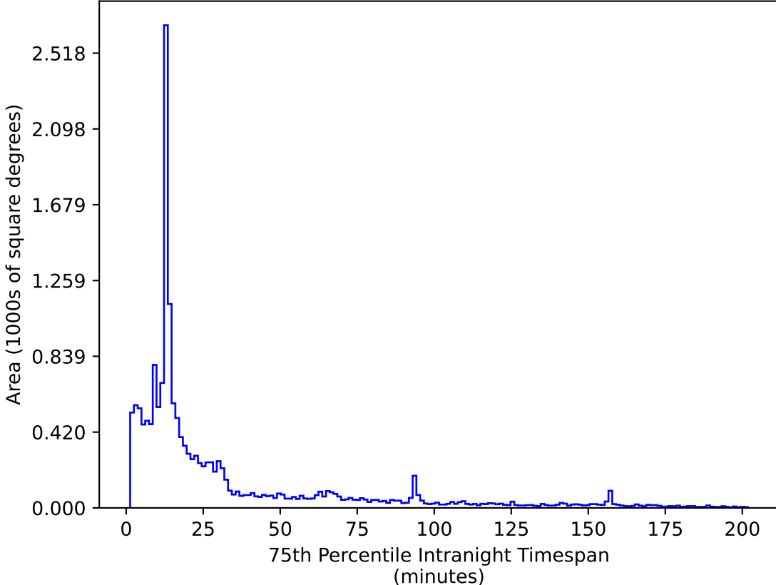
too_ignore_100_4v3.4_10yrs WFD z band: 75th Percentile Intranight Timespan
