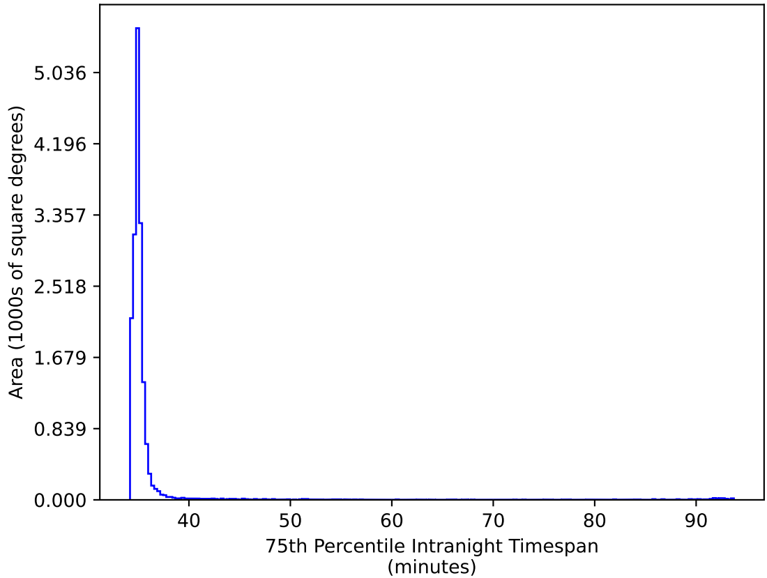
too_ignore_100_4v3.4_10yrs WFD ri bands: 75th Percentile Intranight Timespan
