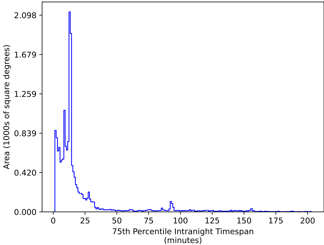
too_ignore_100_4v3.4_10yrs WFD i band: 75th Percentile Intranight Timespan
